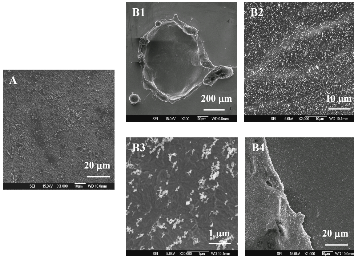
Fig. 3 Picosecond Nd:YAG laser-induced morphology changes of titanium (Scanning Electron Microscopy). Energy density, 10.3 \text{ J/cm}^2 , \lambda_1^{\text{laser}} = 1.064 \text{ }\mu\text{m} ; TEM 00 mode. (A) A view of titanium prior to laser action; (B) titanium after 1 laser pulses action ((1) entire spot, (2,3) center of modified surface at different magnification, and (4) near-periphery of irradiated area).
